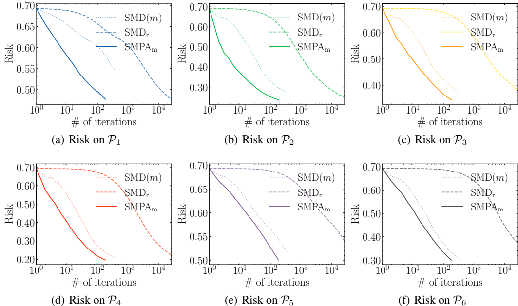
Figure 4: Imbalanced settings with the Adult dataset: individual risk versus the number of iterations
