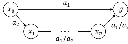
Figure 7: An illustration of state transitions of the constructed hard instance.
