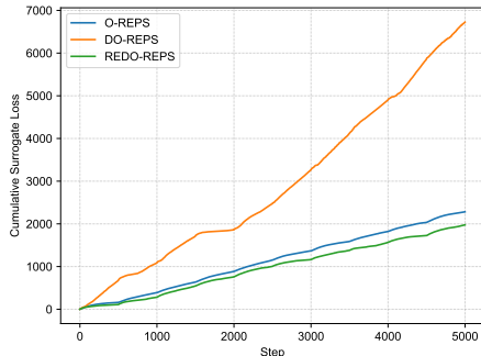
Figure 5: Cumulative surrogate loss
