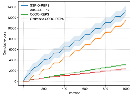
Figure 4: Cumulative loss of algorithms
