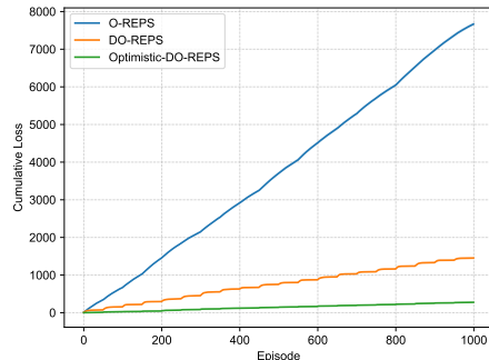
Figure 2: Cumulative loss of algorithms
