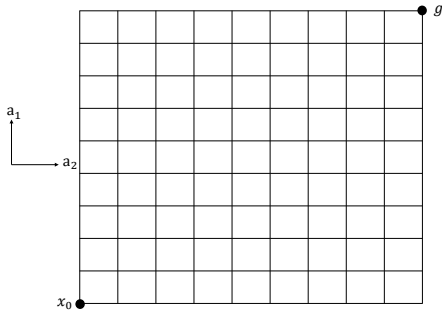
Figure 1: GridWorld environment
