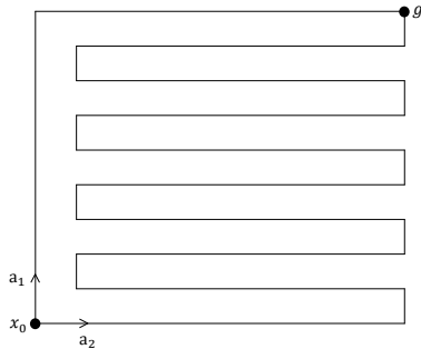
Figure 3: GridWorld environment
