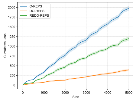
Figure 6: Cumulative loss
