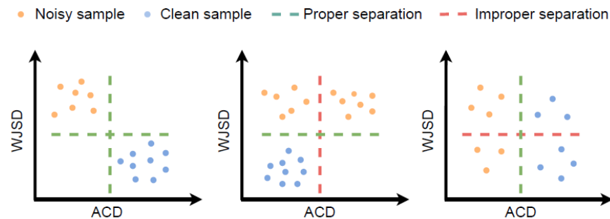
Dimension Selection
