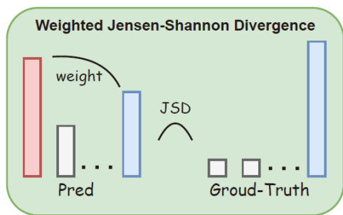
Separation Metrics
