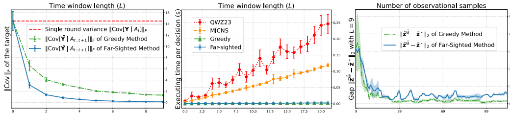
Figure 11: Results on the synthetic dataset, showing the variance reduction w.r.t. the time horizon T , average executing time w.r.t. T , and gap \|\tilde{\mathbf{z}}_t^{\Theta} - \tilde{\mathbf{z}}_t^*\|_2 w.r.t. the number of observational samples N .
