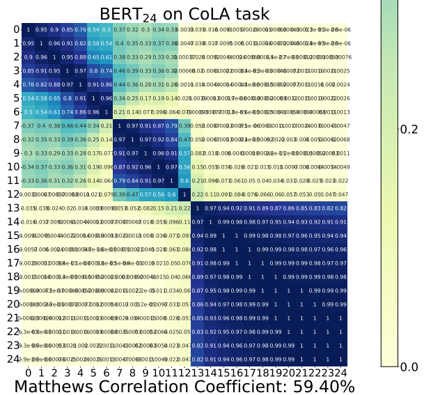
Figure 8: Zoomed-in view of the SVCCA matrix elements for the large BERT model.
