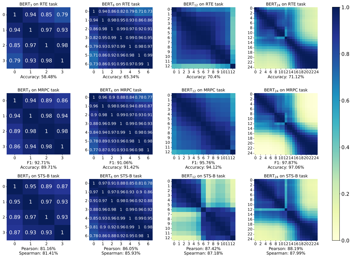
Figure 6: Heatmaps of SVCCA for BERT pre-trained models of varying sizes on several tasks.
