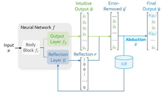
Figure 2: Architecture of Abductive Reflection (ABL-Refl). It replaces the external consistency optimization module with an efficient reflection mechanism, which is abduced directly from \mathcal{KB} .
