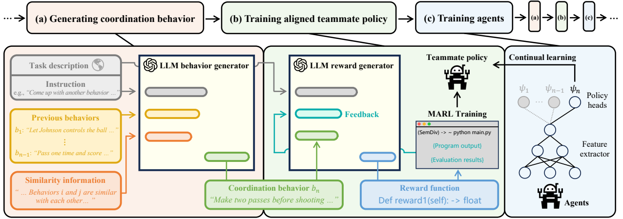
Figure 2. The overall workflow of SEMDIV.
