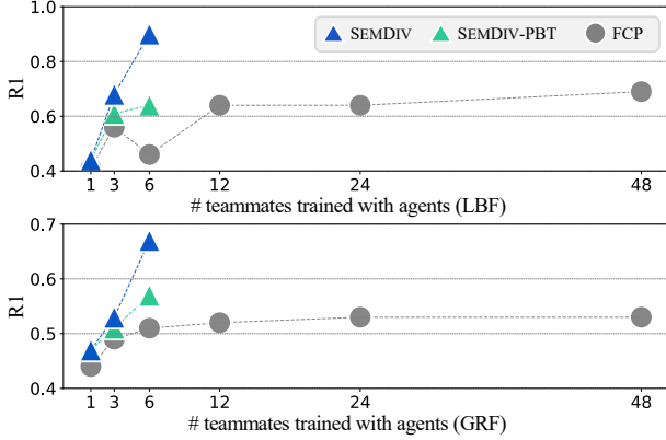
Figure 4. Coordination performance with testing teammates when agents train with various numbers of generated teammates.
