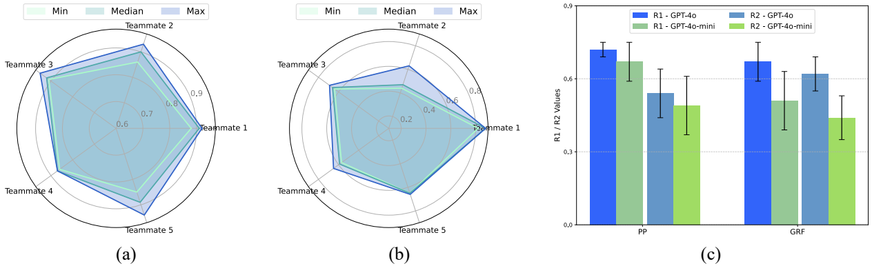
Figure 6. Experiments on the impact of ambiguity in teammates’ coordination behaviors and the quality of LLMs. (a)(b) The minimum, median, and maximum R1 values of each teammate’s 10 different behavior descriptions in LBF and SMACv2. (c) The performance of SEMDIV when using different LLMs in PP and GRF.
