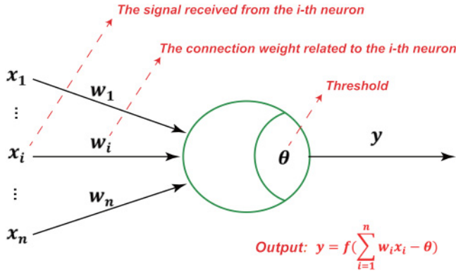
Figure 1: The MP model.
