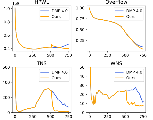
Fig. 5. Optimization iterations for case superblue1 . The blue curve is DREAMPlace 4.0, and the yellow one is our method. Timing optimization of both methods starts from the 500th iteration. TNS and WNS values are converted to their absolute values in the figure for better illustration.
