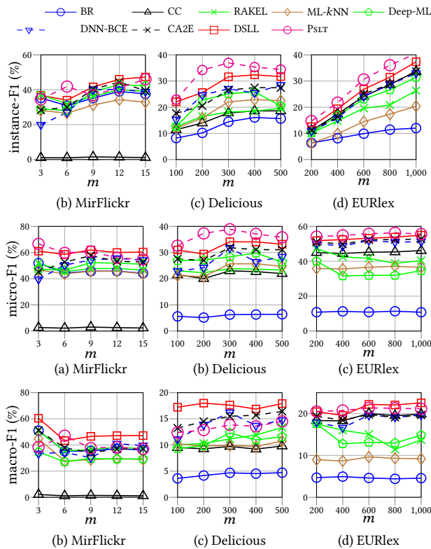
Figure 3: Performance comparison by considering 50% labels as past labels. m indicates the number of new labels.
