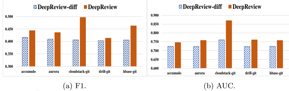
Figure 6: F1 and AUC of the compared methods on five datasets.
