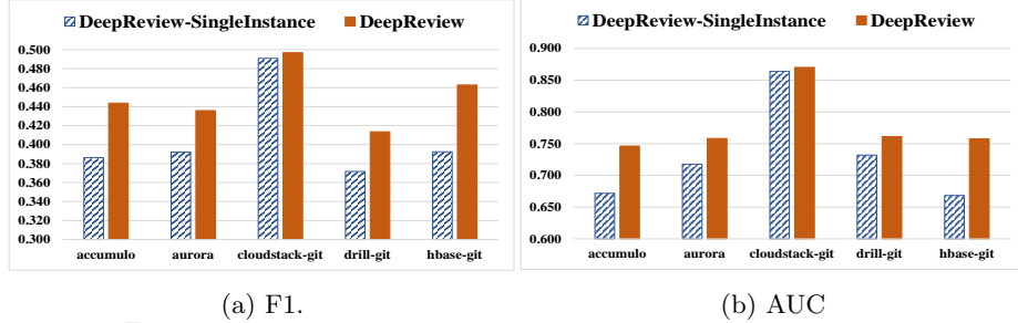
Figure 5: F1 and AUC of the compared methods on five datasets.
