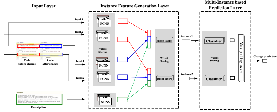
Figure 4: Automatic code review by DeepReview. When a change is processed for prediction, three parts of the change (old code, new code and text descriptions) are firstly encoded as feature vectors to feed into deep model. Then three parts of convolutional neural networks are followed to extract semantic features for source code and text description separately. After that a fully-connected network is used to get fusion feature for hunks. Finally, another fully-connected network and a max-pooling layer is connected to generate a prediction indicating approved or rejected of the change.
