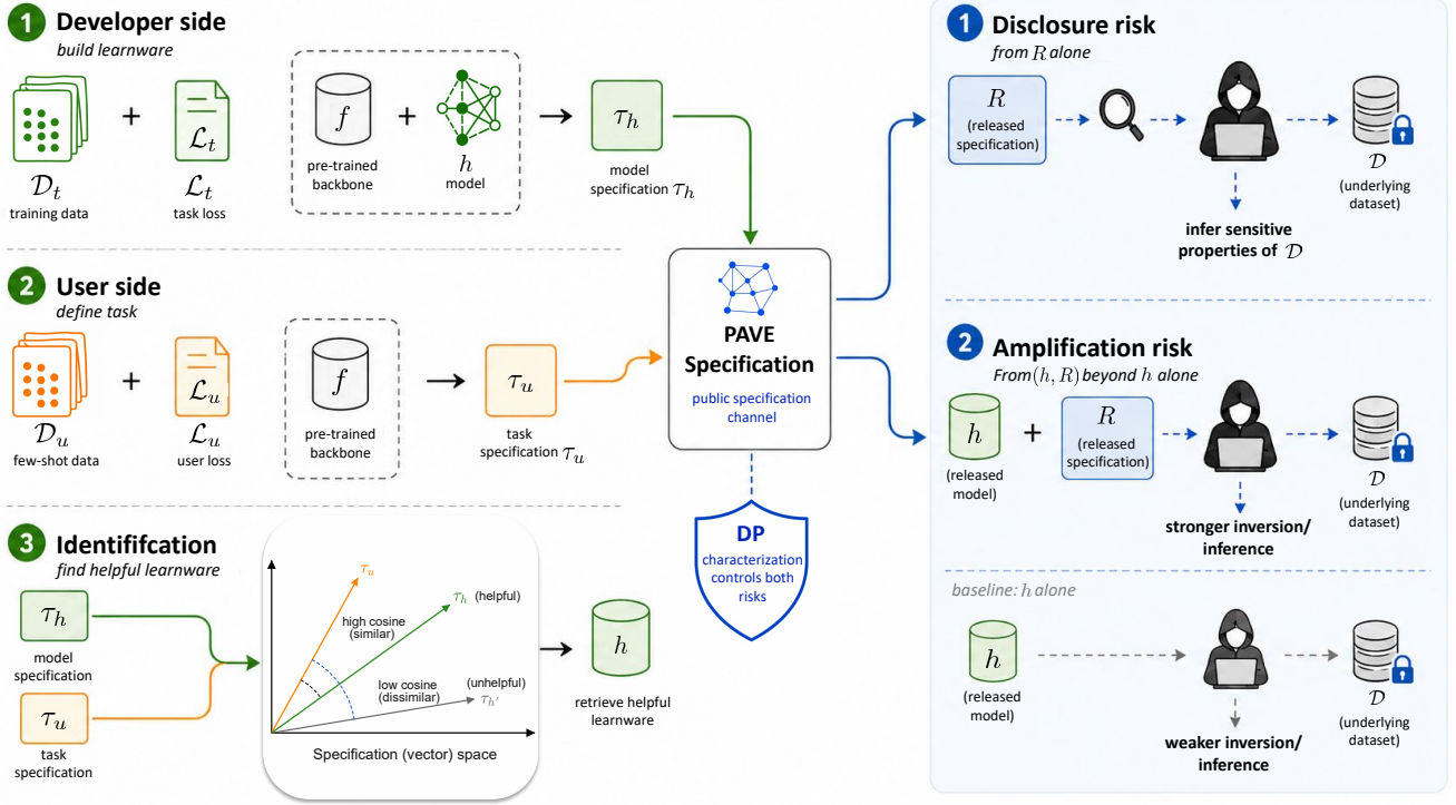
Figure 1: Overview of PAVE-based learnware identification and reuse and specification-induced privacy risks.
