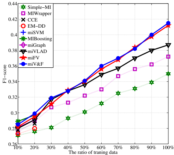
Figure 7. Macro-averaged F-score results of TRECVID 2005. Note that, when the ratio of training data is bigger than 20%, CCE, EM-DD, miSVM, MIBoosting and miGraph can not return results in 48 hours. This figure is best viewed in color.
