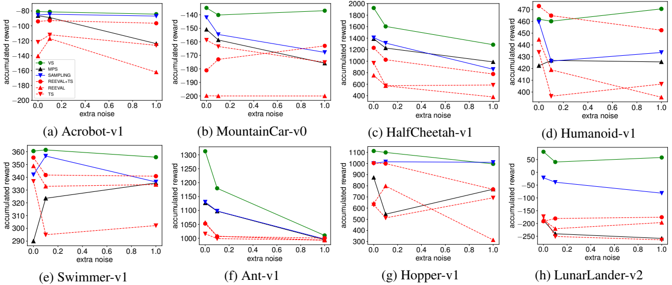
Figure 2: Comparison of the performance under extra noises of 0, 0.1, and 1 times of the noise level respectively
