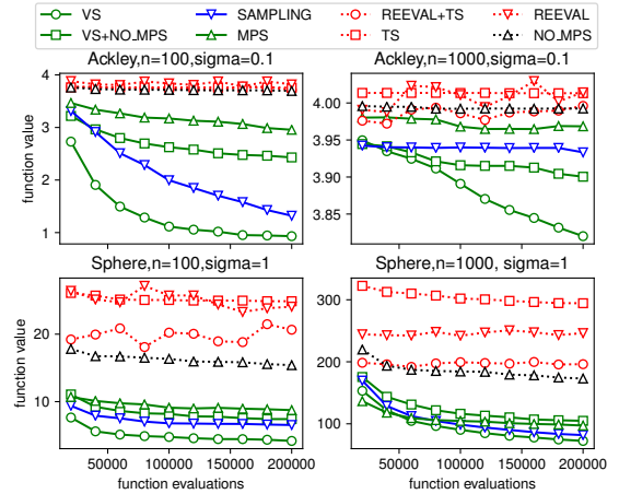
Figure 1: The function value of each noise handling mechanism during the optimization process. For Ackley function, we set the dimension size n = 100 and 1000 , the standard deviation of noise \sigma = 0.1 . For Sphere function, we set the dimension size n = 100 and 1000 , the standard deviation of noise \sigma = 1 .
