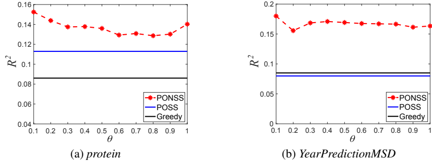
Figure 2: Sparse regression with the budget k = 14 ( R^2 : the larger the better): the comparison between PONSS with different \theta values, POSS and the greedy algorithm.
