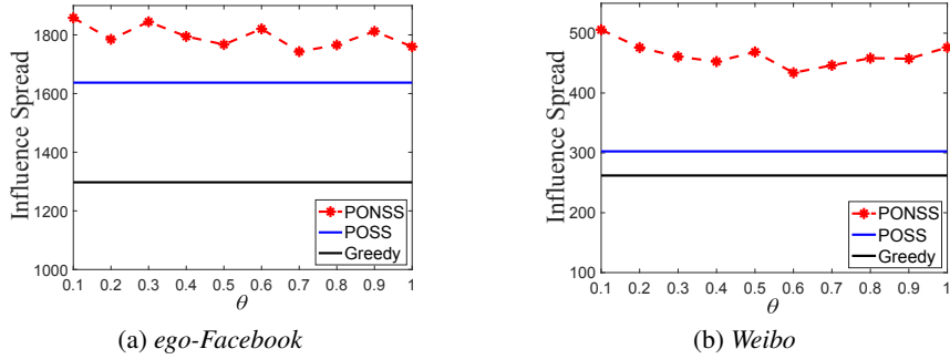
Figure 1: Influence maximization with the budget k = 7 (influence spread: the larger the better): the comparison between PONSS with different \theta values, POSS and the greedy algorithm.
